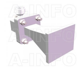
LB-90-10-C-NFSP Standard Gain Horn Antenna 8.2-12.4GHz 10dB Gain N Type Female
