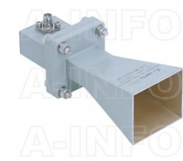
LB-90-10-C-SF Standard Gain Horn Antenna 8.2-12.4GHz 10dB Gain SMA Female
