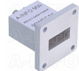
90WECAM Endlaunch Rectangular Waveguide to Coaxial Adapter 8.2-12.4GHz WR90 to 2.92mm Female
